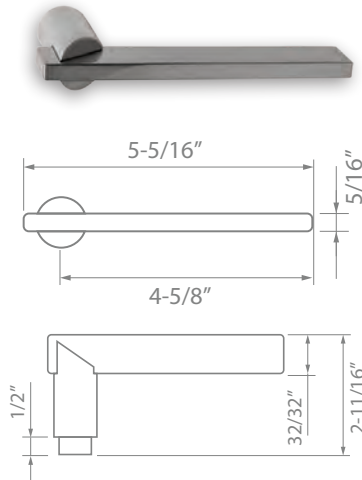
943 RALEIGH LEVER
