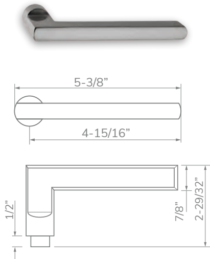
939 CHARLOTTE LEVER
