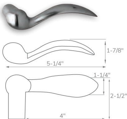
909 COLUMBUS LEVER
