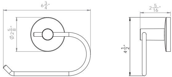
Paper Holder
